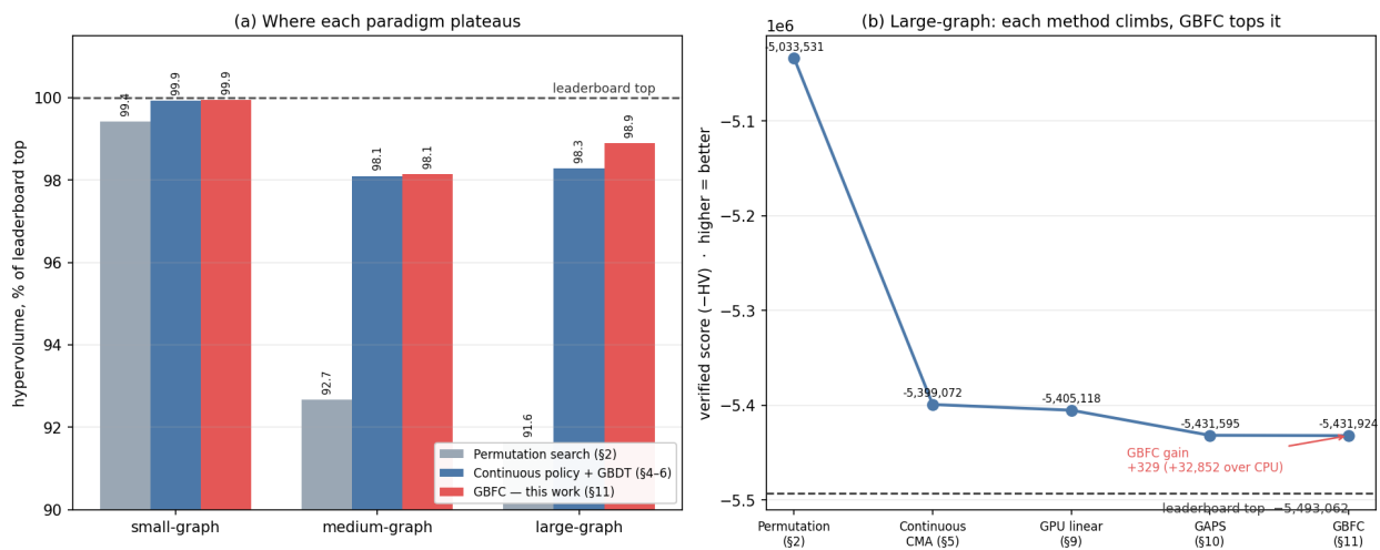
Figure 11: (a) Hypervolume as a percentage of the leaderboard top, by method and instance: direct permutation search (§2), the continuous policy with GBDT (§4–6), and GBFC (this work, §11). (b) The large-graph score climbing through each method — permutation → continuous CMA → GPU-linear → GAPS → GBFC — toward the leaderboard top (dashed) and the certified near-optimal ceiling.
