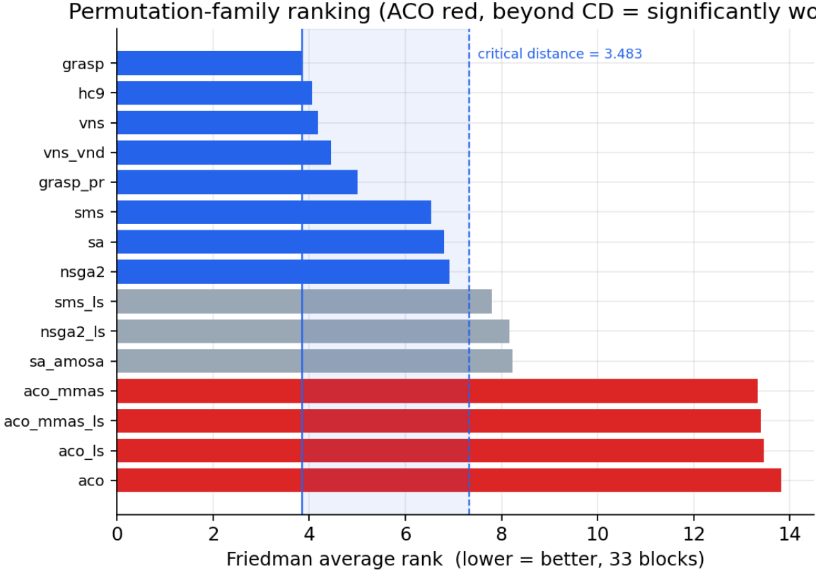
Figure 1: Friedman average ranks of the permutation-space families. GRASP leads; the four ACO variants sit beyond the critical distance and are significantly worse.
