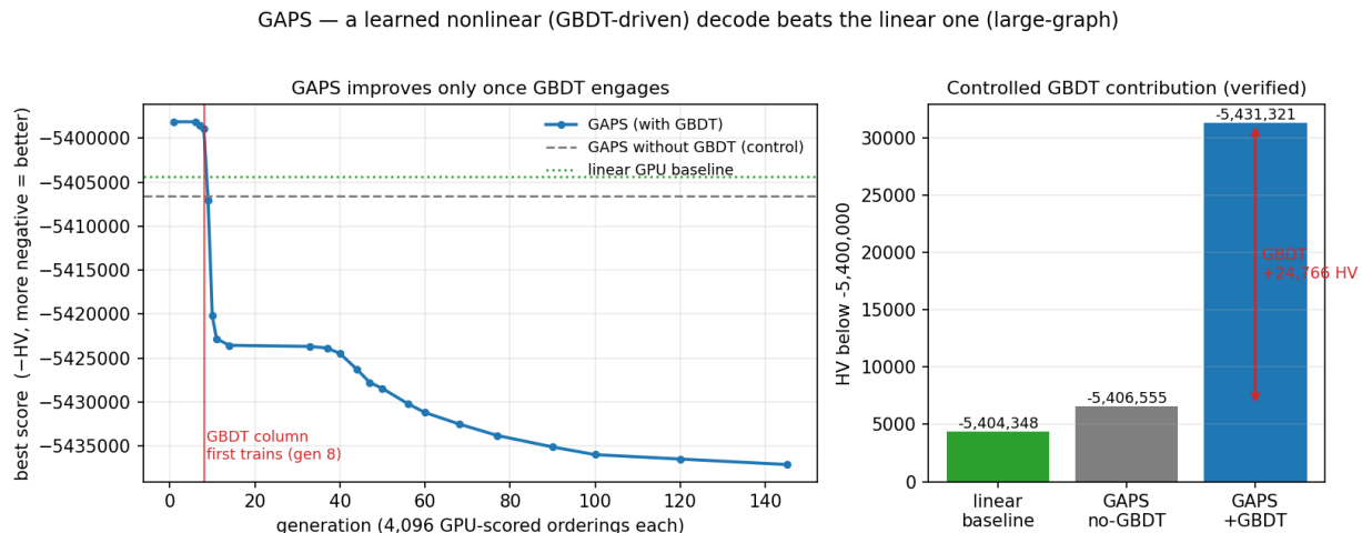
Figure 10: Left: the with-GBDT GAPS trajectory (Tesla T4, seed 42, warm-started from the banked portfolio) is flat until generation 8 — the first GBDT retrain — then breaks loose, the improvement time-locked to the GBDT mechanism engaging; the dashed/dotted lines are the GBDT-disabled control and the linear baseline. Right: the verified official top-20 scores; the gap between GAPS-with-GBDT and the GBDT-disabled control is the controlled GBDT contribution, +24,766 HV .
